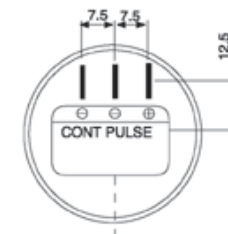
Bottom View 5
