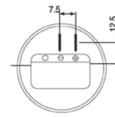
Bottom View 4
