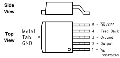
Surface Mount Package 5-Lead TO-263 (S)
