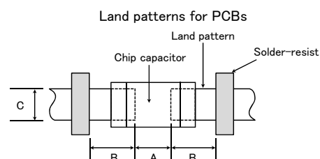
Chip capacitor
