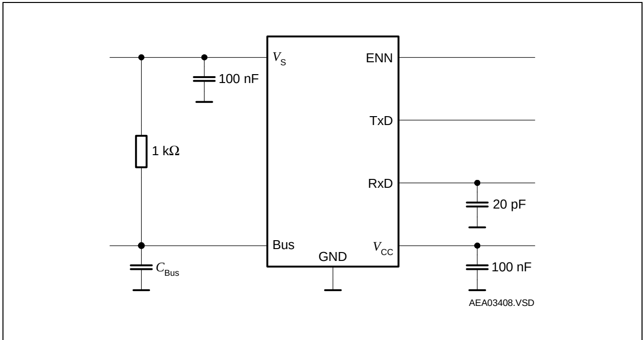
Figure 4 Test Circuits
