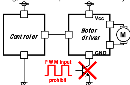
Fig. 51 GND line PWM switching prohibited
