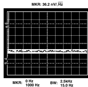
TPC 18. Voltage Noise Density, V_S = +3\text{ V to } \pm 5\text{ V}, A_{VO} = 1000
