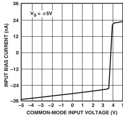
TPC 41. Input Bias Current vs. Common-Mode Voltage, V_S = \pm 5V
