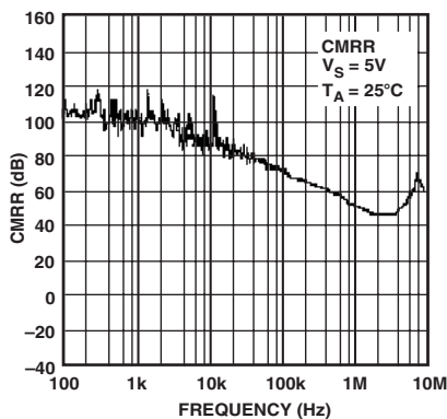
TPC 29. CMRR vs. Frequency, V_S = 5\text{ V}
