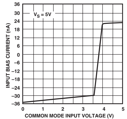
TPC 24. Input Bias Current vs. Common-Mode Input Voltage, V_S = 5\text{ V}
