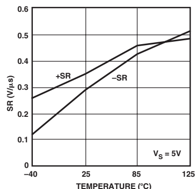
TPC 32. OP291 Slew Rate vs. Temperature, V_S = 5\text{ V}
