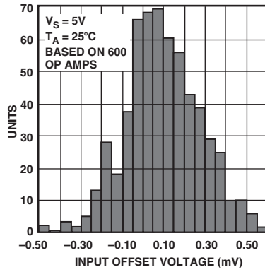
TPC 19. OP291 Input Offset Voltage Distribution, V_S = 5\text{ V}
