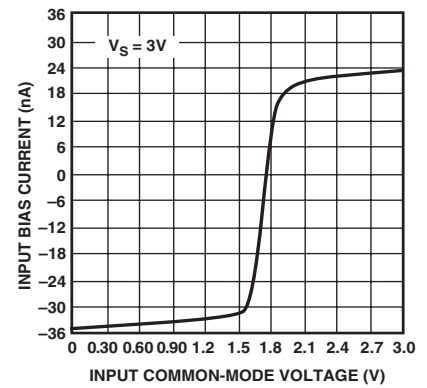
TPC 6. Input Bias Current vs. Input Common-Mode Voltage, V_S = 3\text{ V}
