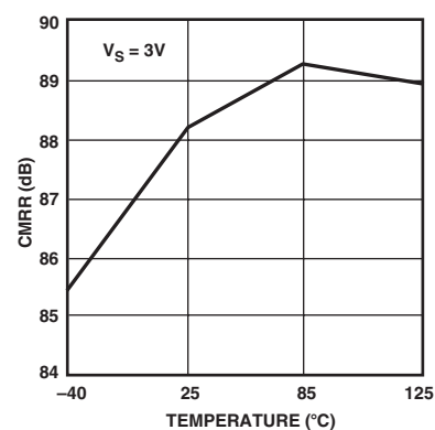
TPC 12. CMRR vs. Temperature, V_S = 3\text{ V}
