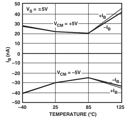
TPC 39. Input Bias Current vs. Temperature, V_S = \pm 5V
