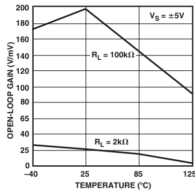
TPC 44. Open-Loop Gain vs. Temperature, V_S = \pm 5V
