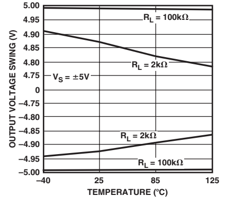
TPC 42. Output Voltage Swing vs. Temperature, V_S = \pm 5V
