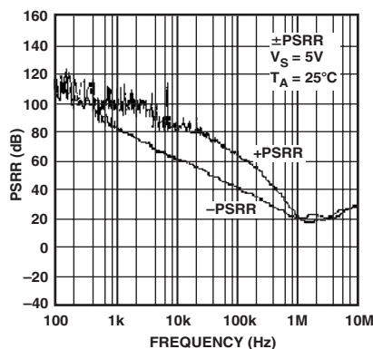
TPC 31. PSRR vs. Frequency, V_S = 5\text{ V}
