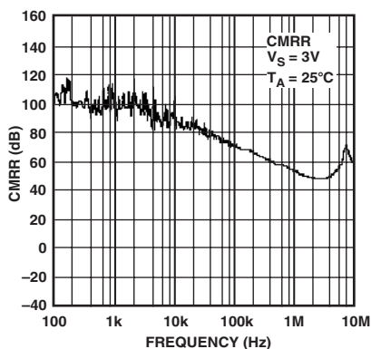
TPC 11. CMRR vs. Frequency, V_S = 3\text{ V}
