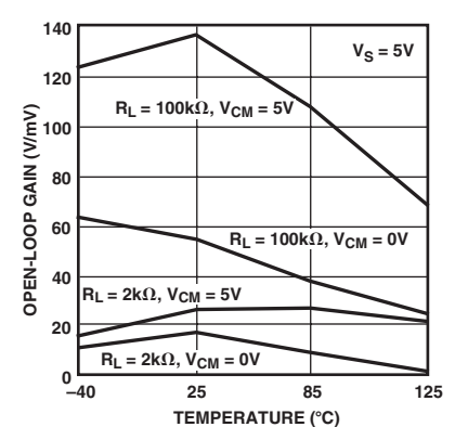
TPC 27. Open-Loop Gain vs. Temperature, V_S = 5\text{ V}
