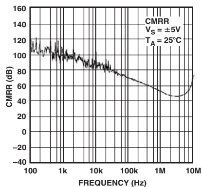
TPC 46. CMRR vs. Frequency, V_S = \pm 5\text{ V}
