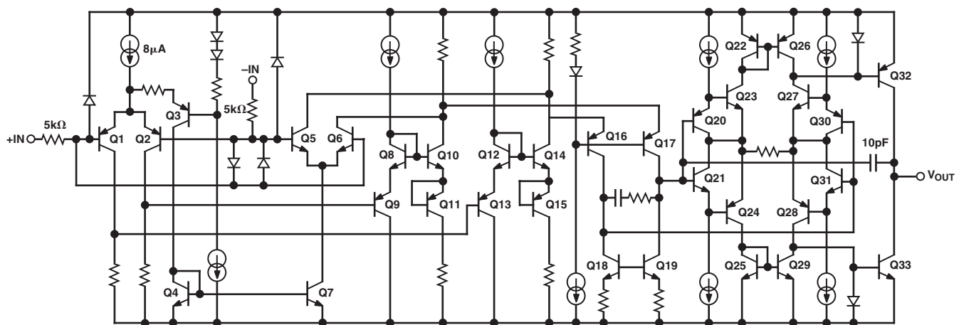
Figure 2. Simplified Schematic
