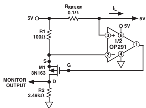
Figure 10. A High-Side Load Current Monitor
