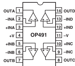
14-Lead PDIP
