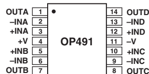
14-Lead TSSOP
