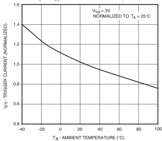
Fig. 4 Trigger Current vs. Ambient Temperature
