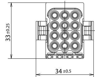
Plug, 12 poles
