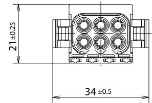
Plug, 6 poles
