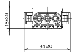
Plug, 3 poles
