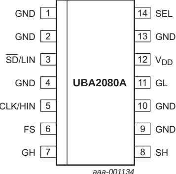
Fig 4. UBA2080A: Pin configuration SO14 package
