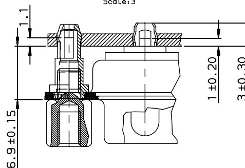
DETAIL OF PRESS FIT Scale:3
