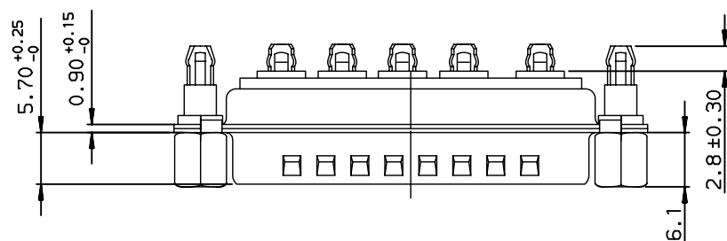
LAYOUT DIMENSIONS (after plating) CONNECTOR SIDE VIEW
