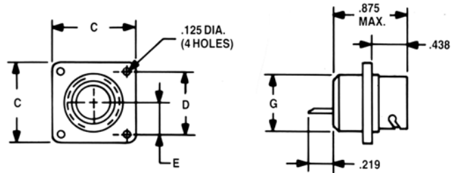
Panel Receptacle
