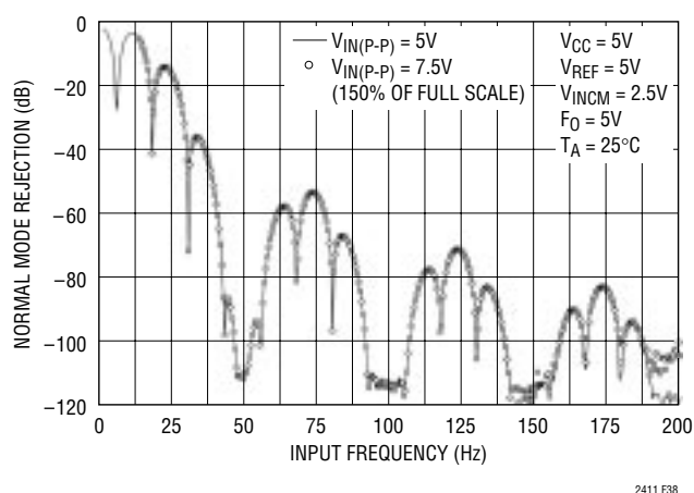
Figure 38. Measured Input Normal Mode Rejection vs Input Frequency (LTC2411)
