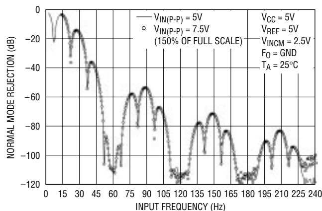
Figure 37. Measured Input Normal Mode Rejection vs Input Frequency (LTC2411)
