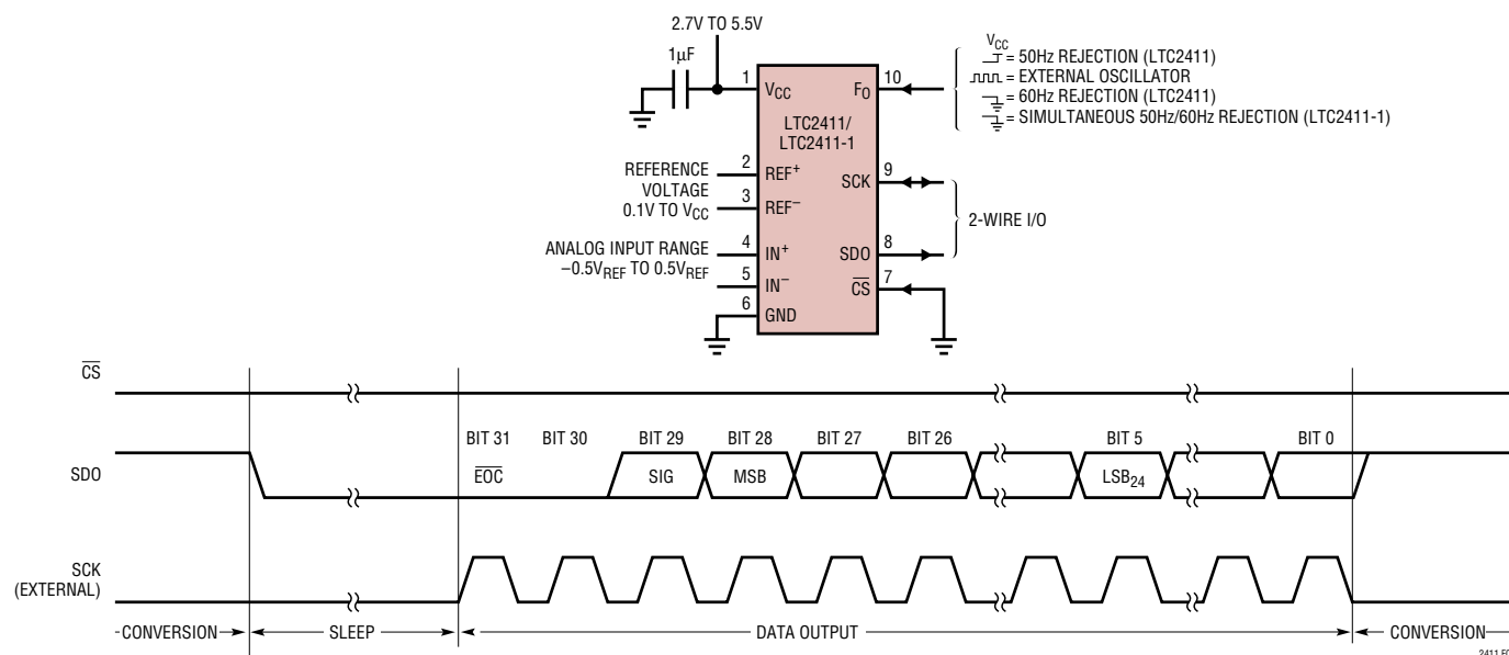
Figure 7. External Serial Clock, \overline{\text{CS}} = 0 Operation
