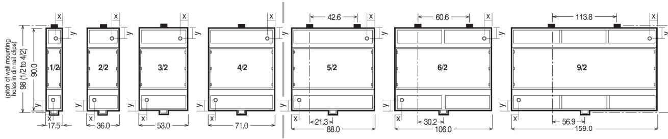
Single Row Terminals/ covers on one side
