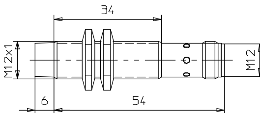
E2EL-X4M□-M1L
