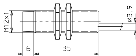
E2EL-X4M□-L
