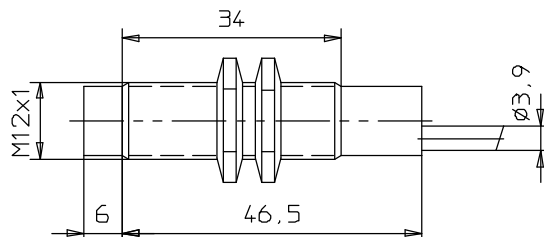
E2EL-X4M□-L
