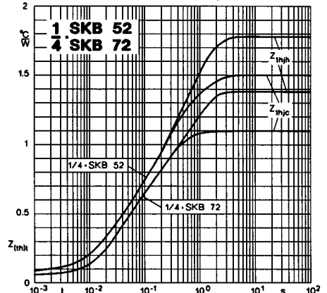
Fig. 12 a Transient thermal impedance vs. time
