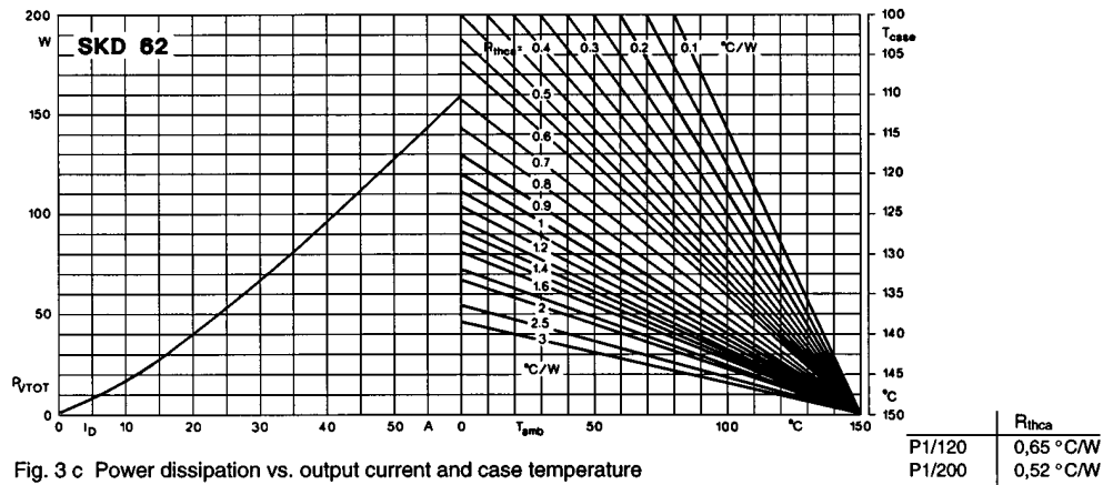
Fig. 3 c Power dissipation vs. output current and case temperature
