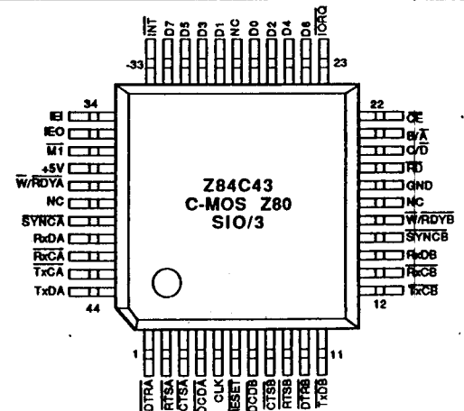
Figure 7b. 44-Pin LOFP Pin Assignments
