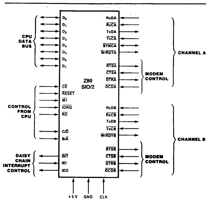
Figure 1. Pin Functions
