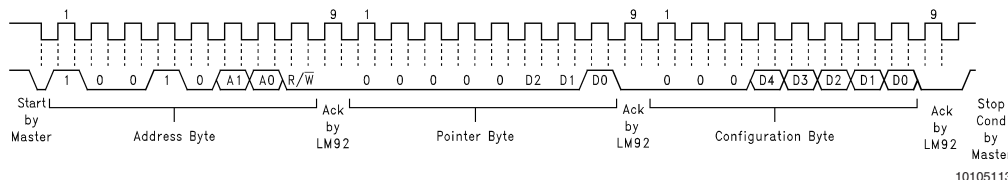
Configuration Register Write
