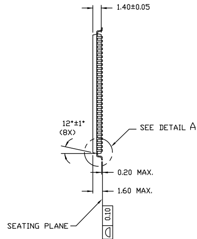
Figure 10. 100-pin TQFP (14 × 20 × 1.4 mm) A100RA Package Outline, 51-85050
