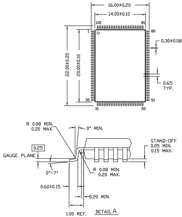
Figure 10. 100-pin TQFP (14 × 20 × 1.4 mm) A100RA Package Outline, 51-85050
