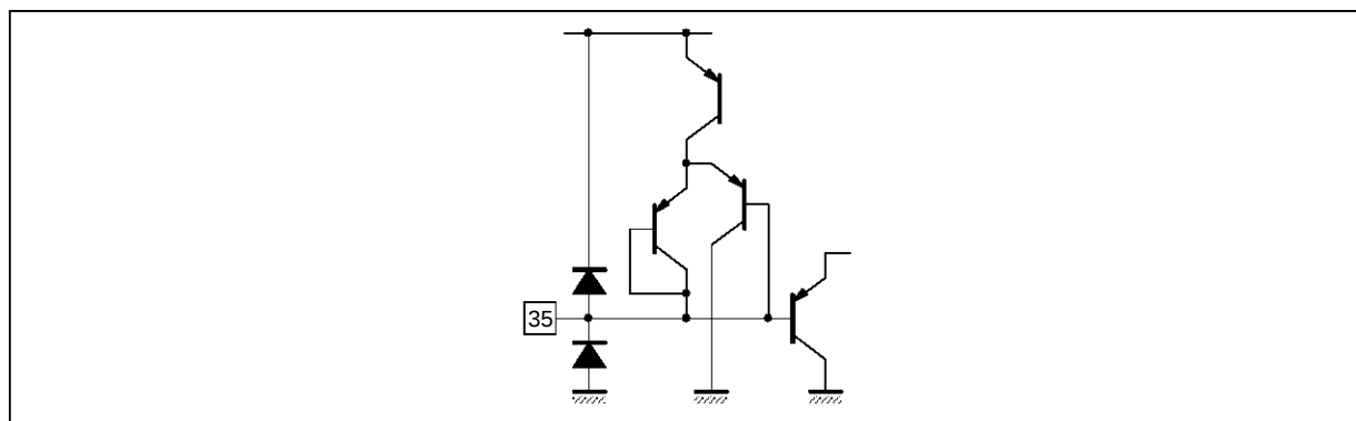
Figure 27 : Pin 35 (FBL)
