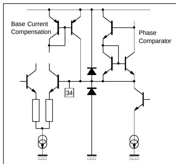
Figure 26 : Pin 34 (CLPF)
