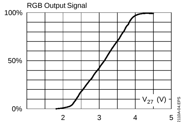
Figure 2 : Saturation Control Curve
