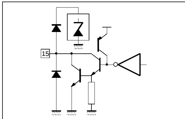
Figure 13 : Pin 15 (HOUT)
