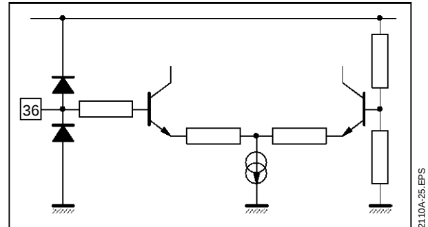
Figure 23 : Pin 36 (BRIG)
