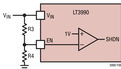
Figure 6. Enable
