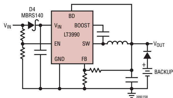
Figure 8. Diode D4 Prevents a Shorted Input from Discharging a Backup Battery Tied to the Output. It Also Protects the Circuit from a Reversed Input. The LT3990 Runs Only when the Input is Present
