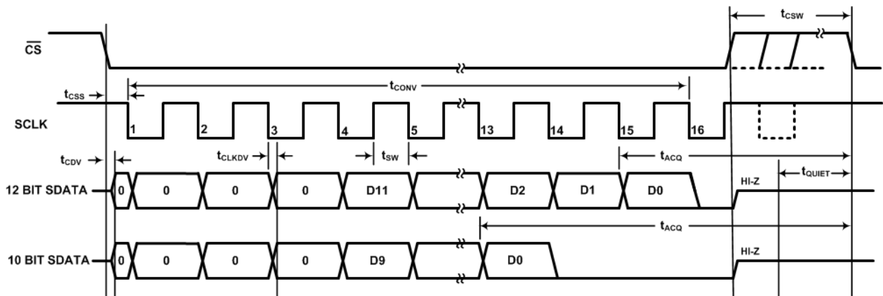
FIGURE 3. SERIAL INTERFACE TIMING DIAGRAM
