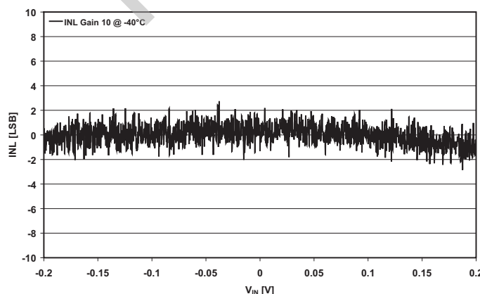
Figure 33. INL -40°C
