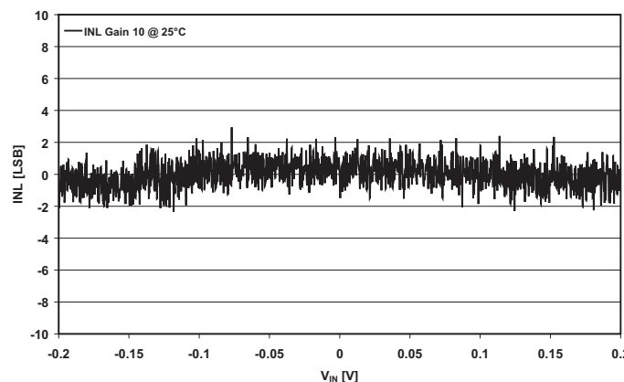
Figure 34. INL 25°C
