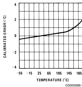
Calibrated Error
