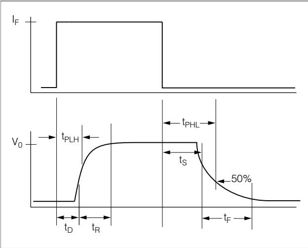
Figure 3. Non-saturated switching timing
