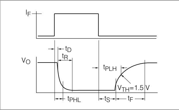
Figure 4. Saturated switching timing
