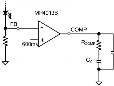
Figure 5: Compensation Network
