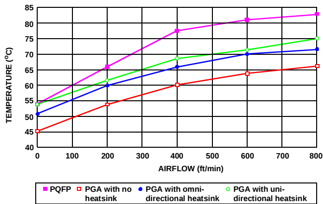
Figure 25. 25 MHz Maximum Allowable Ambient Temperature
