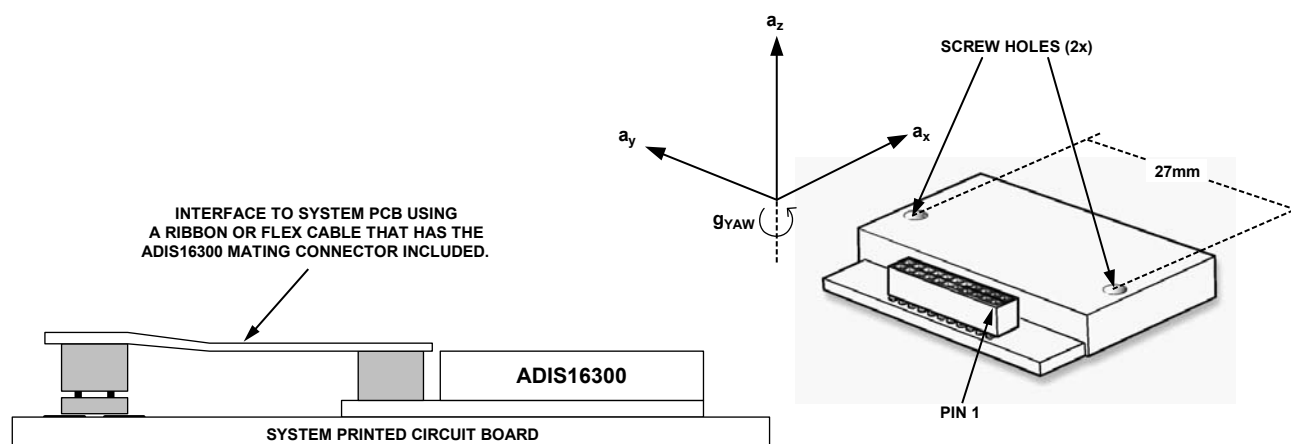
Figure 5. Pin Configuration
