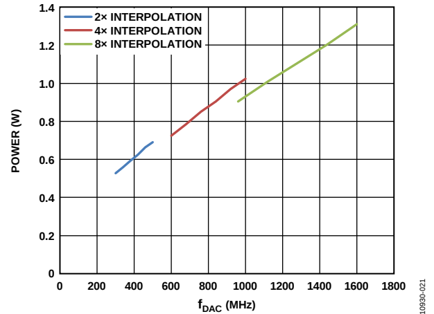
Figure 24. Total Power Consumption vs. f_{DAC} over Interpolation
