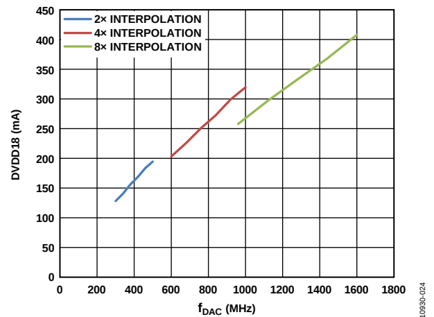
Figure 25. DVDD18 Current vs. f_{DAC} over Interpolation
