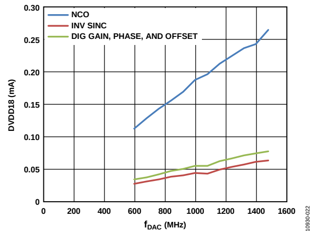
Figure 26. DVDD18 Current vs. f_{DAC} over Digital Functions
