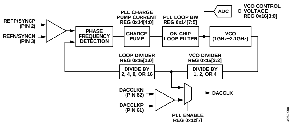
Figure 52. PLL Clock Multiplication Circuit
