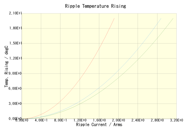
C3225X7R1H225K200AB(100kHz) C3225X7R1H225K200AB(500kHz) C3225X7R1H225K200AB(1MHz)
