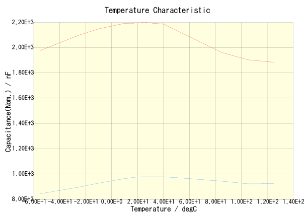
C3225X7R1H225K200AB(DC Bias = 0V) C3225X7R1H225K200AB(DC Bias = 25V)
