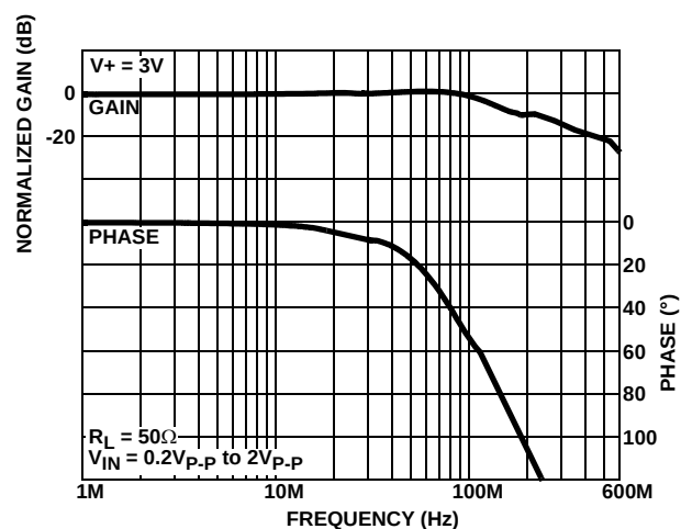
FIGURE 19. FREQUENCY RESPONSE
