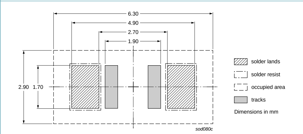
Fig 8. Wave soldering footprint SOD80C
