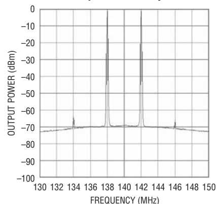
2-Tone Spectrum Analyzer Plot
