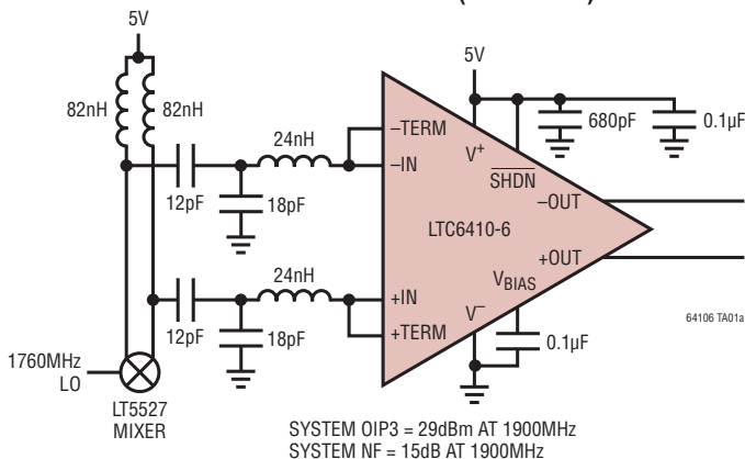
Post Mixer Gain Block (140MHz IF)
