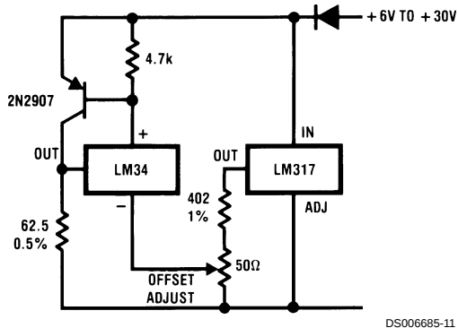
4-to-20 mA Current Source (0 to +100°F)
