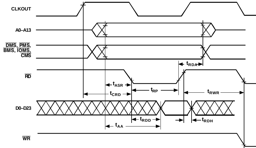
Figure 27. Memory Read
