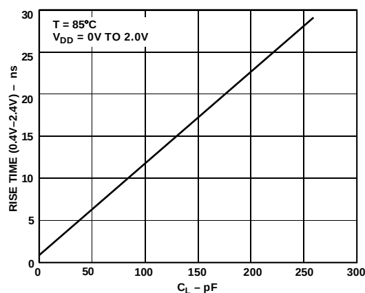
Figure 22. Typical Output Rise Time vs. Load Capacitance (at Maximum Ambient Operating Temperature)
