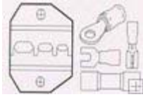
Die for Barrel Type Connectors 22-10 AWG Insulated
