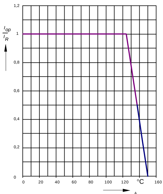
Current derating I_{op} // R versus ambient temperature T_A
