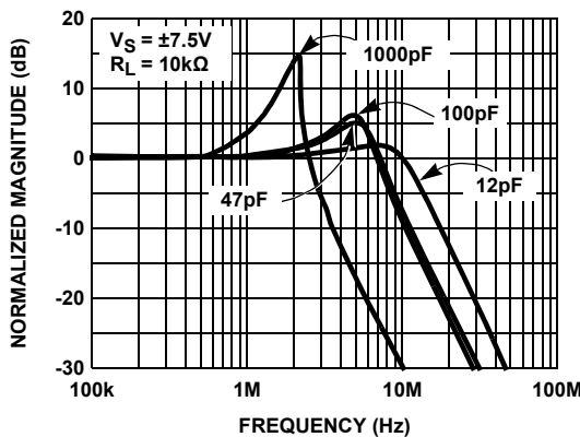
FIGURE 2. FREQUENCY RESPONSE FOR VARIOUS C_L (Buffer)
