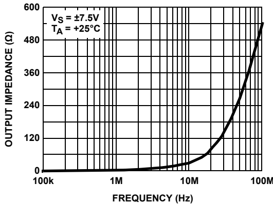
FIGURE 4. OUTPUT IMPEDANCE vs FREQUENCY (BUFFER)
