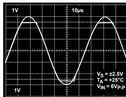
FIGURE 22. Operation with Beyond-the-Rails Input
