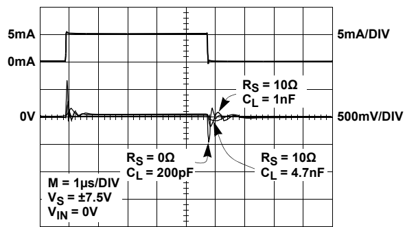
FIGURE 12. TRANSIENT LOAD REGULATION - SINKING (BUFFER)
