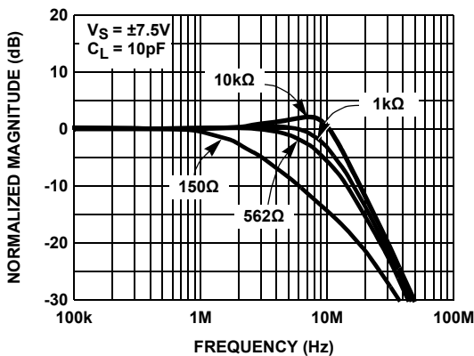
FIGURE 1. FREQUENCY RESPONSE FOR VARIOUS R_L (BUFFER)
