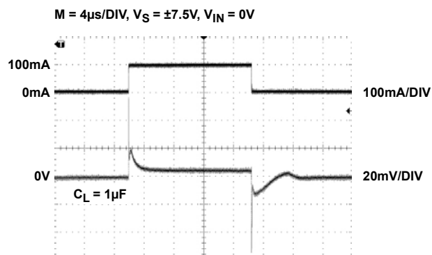
FIGURE 14. TRANSIENT LOAD REGULATION - SINKING ( V_{COM} )
