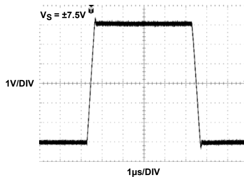
FIGURE 16. LARGE SIGNAL TRANSIENT RESPONSE (BUFFER)
