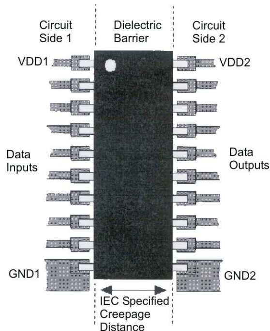
Figure 14. Creepage Distance
