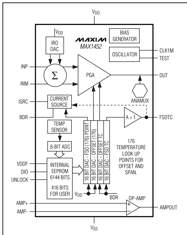
Figure 1. Functional Diagram
