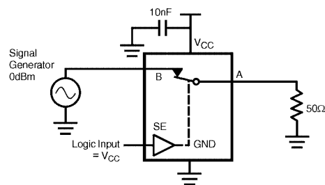
FIGURE 5. Crosstalk
