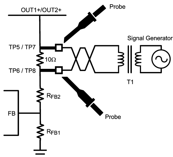
Figure 10. Loop Response Measurement Setup
