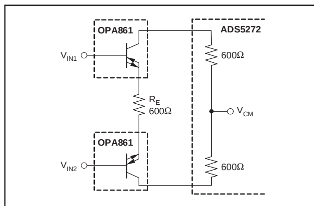
Figure 48. High CMRR, Moderate Precision, Differential I/O ADC Driver
