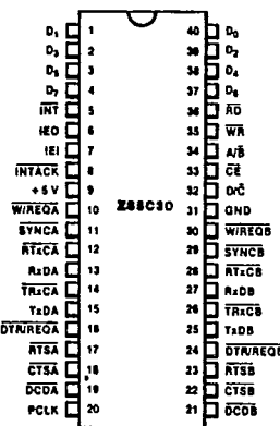
Figure 1a. Pin Functions, Z85C30
