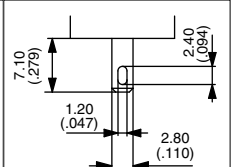
Quick-connect Z
