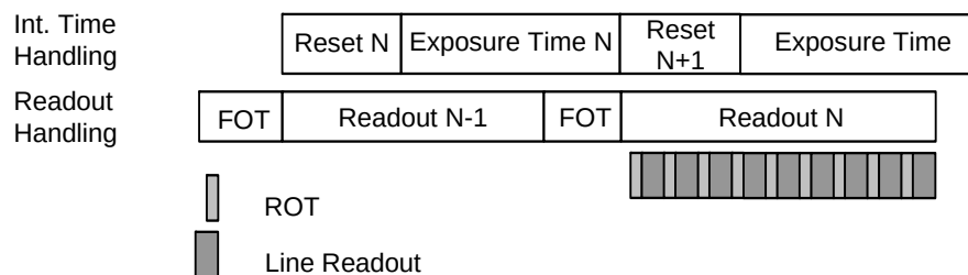
Figure 12. Integration and Readout for Pipelined Shutter
