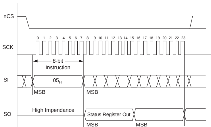
Figure 9-35. RDSR Operation Sequence
