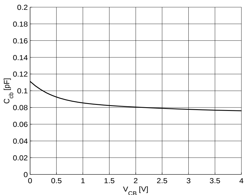
Figure 5-9 Collector Base Capacitance C_{CB} = f(V_{CB}) , f = 1 MHz
