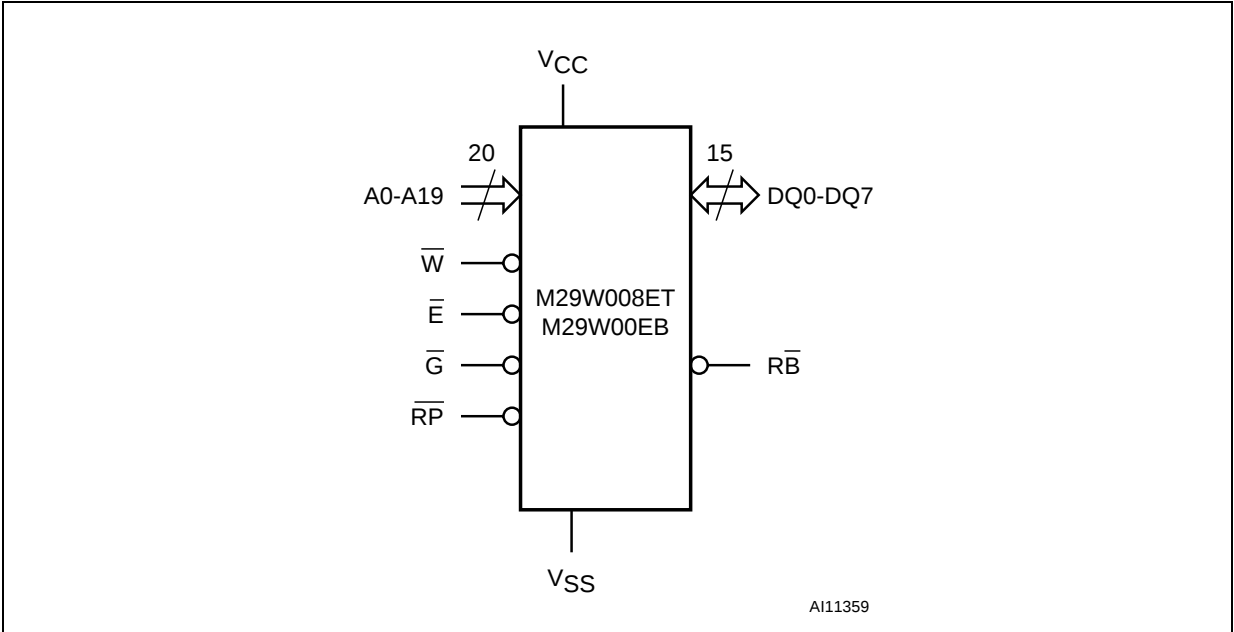
Figure 2. Logic diagram
