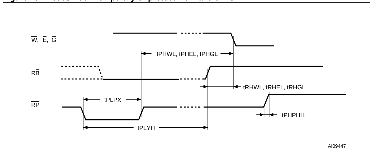
Figure 13. Reset/Block Temporary Unprotect AC Waveforms
