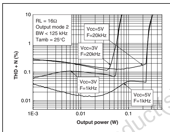
Figure 7: HDout THD+N vs. output power (output mode 2)
