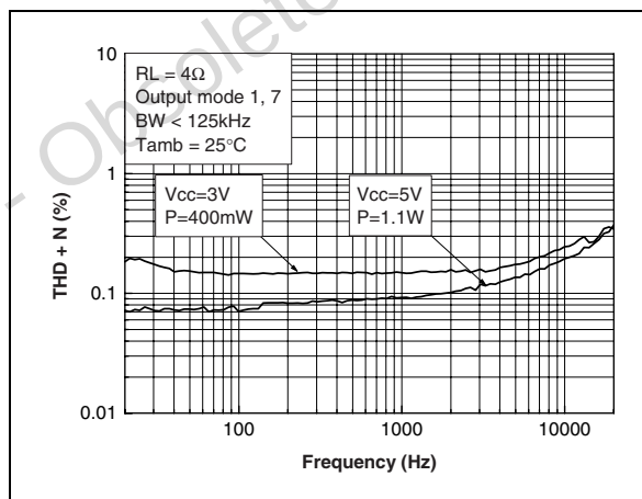
Figure 14: Spkout THD+N vs. frequency (output modes 1, 7)
