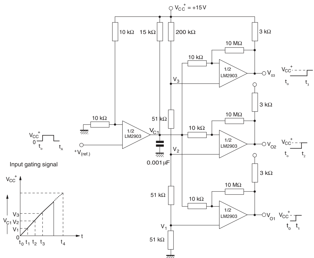
Figure 20. Time delay generator
